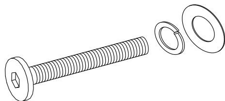
ALLEN KEY BOLT: M6 X 70mm - QTY 8 LOCK WASHER: \varnothing 10 / \varnothing 6 X 1.5mm - QTY 8 WASHER: \varnothing 16 / \varnothing 6 X 1mm - QTY 8 QTY 8 SETS
