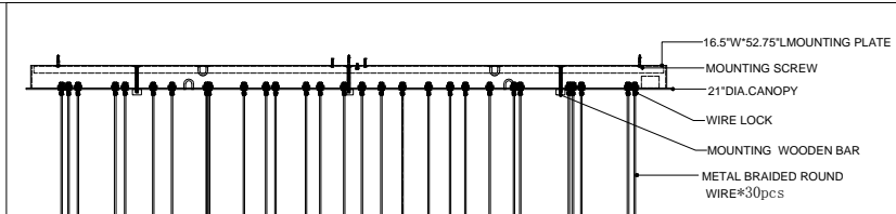
CANOPY DETAIL
