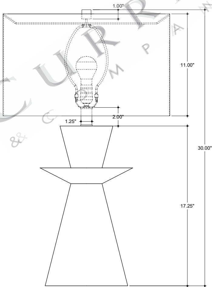
FRONT VIEW
