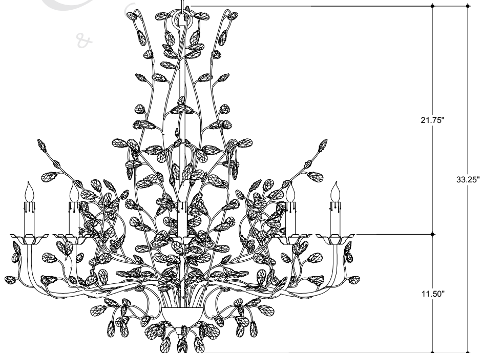
FRONT VIEW
