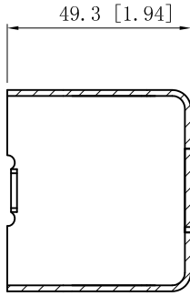
CUTAWAY VIEW A-A
