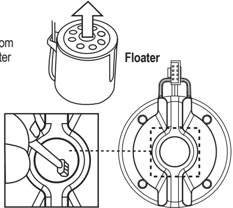
Looking down inside of floater at ultrasonic disc.
