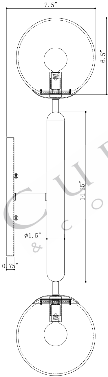
SIDE VIEW
