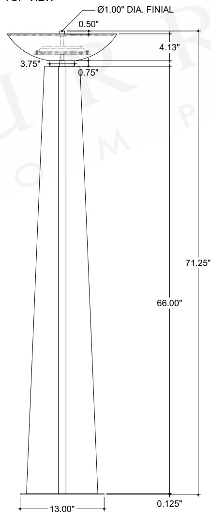
FRONT VIEW
