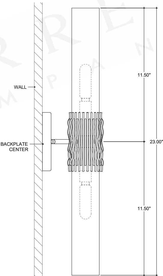
SIDE VIEW
