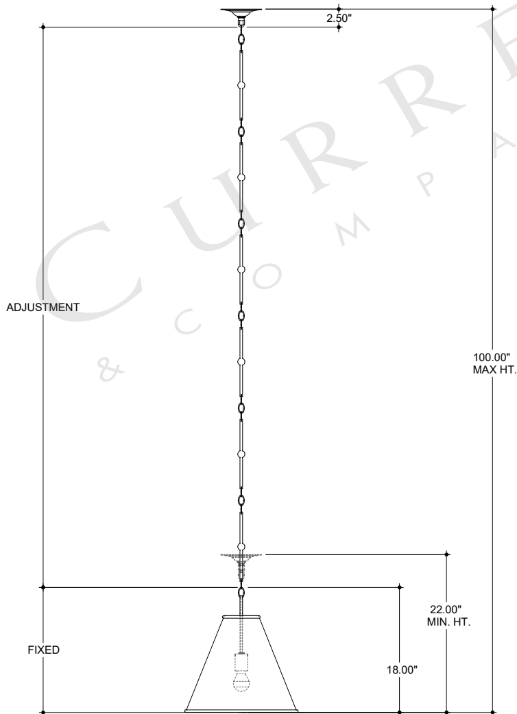
FRONT VIEW
