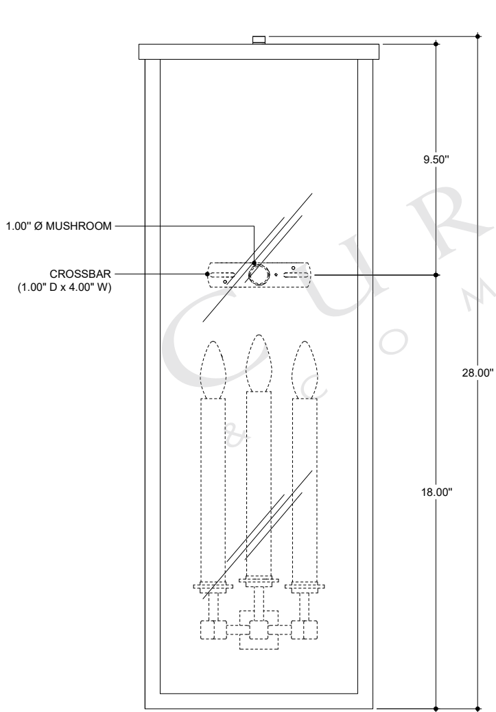
FRONT VIEW
