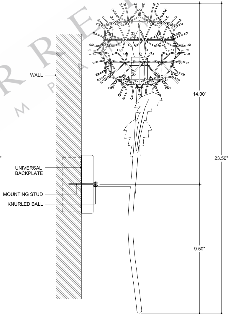
SIDE VIEW
