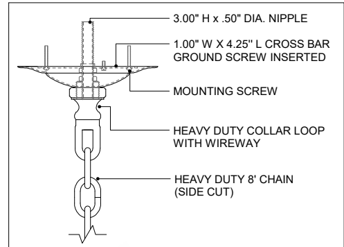
CANOPY DETAIL
