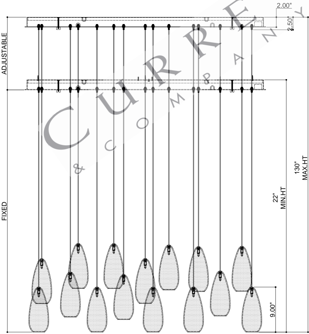
FRONT VIEW
