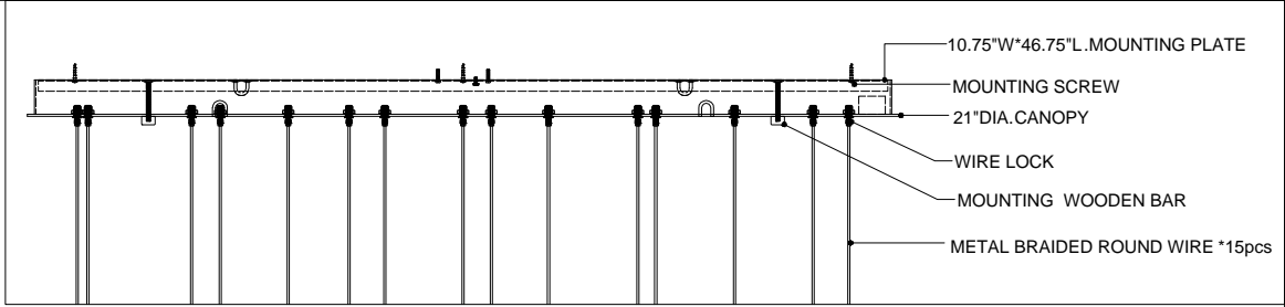
CANOPY DETAIL
