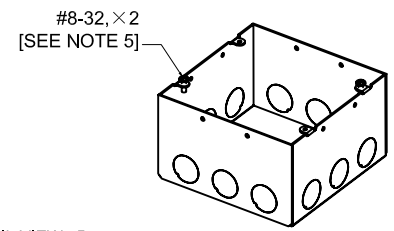
WELDING STYLE DETAIL VIEW B
