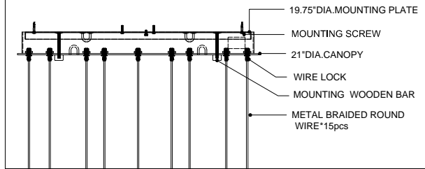
CANOPY DETAIL
