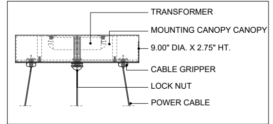
CANOPY DETAIL
