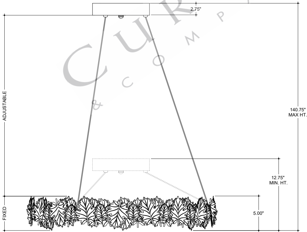
FRONT VIEW
