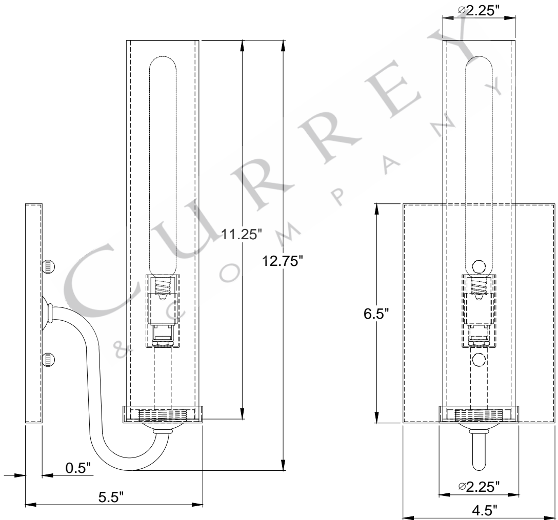
SIDE VIEW
