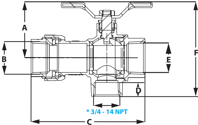
Hot/Cold/Recirculation Valve
