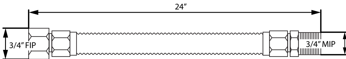
Gas Connector
