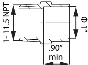
Sweat Adapter
