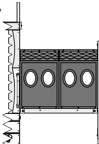
Fig. 47.2 Side View
