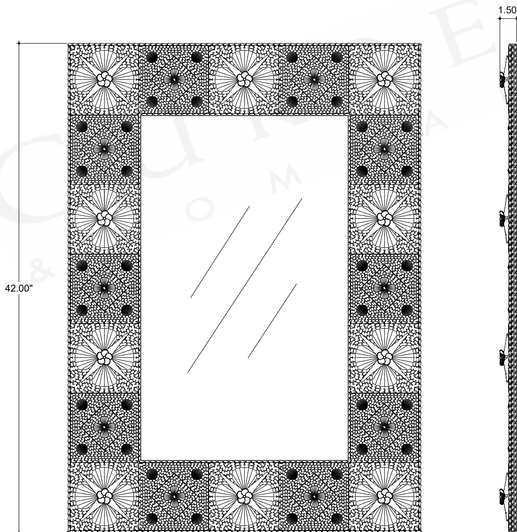
FRONT VIEW
