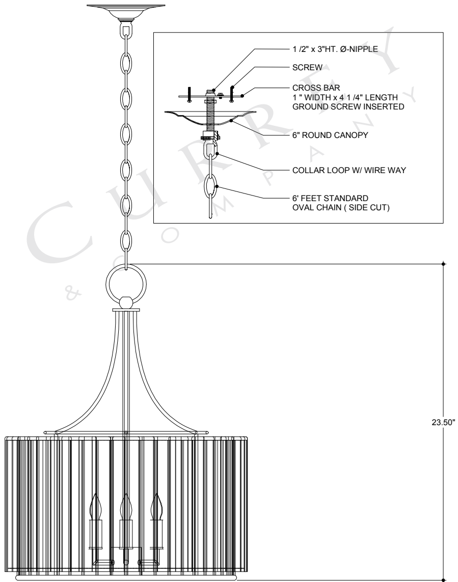
FRONT VIEW
