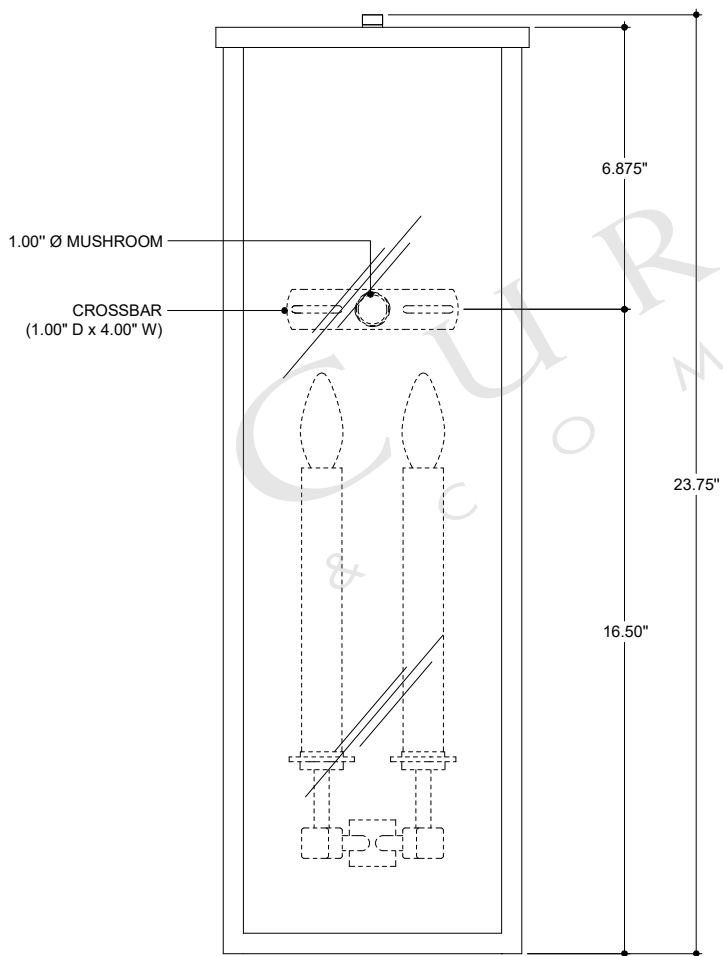
FRONT VIEW
