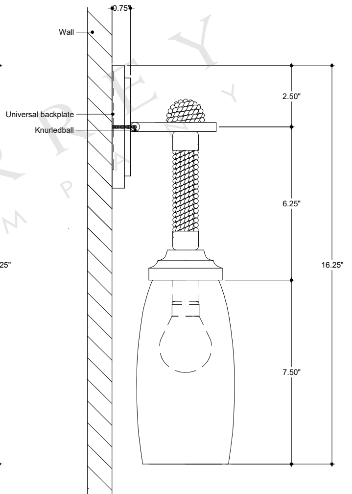
SIDE VIEW
