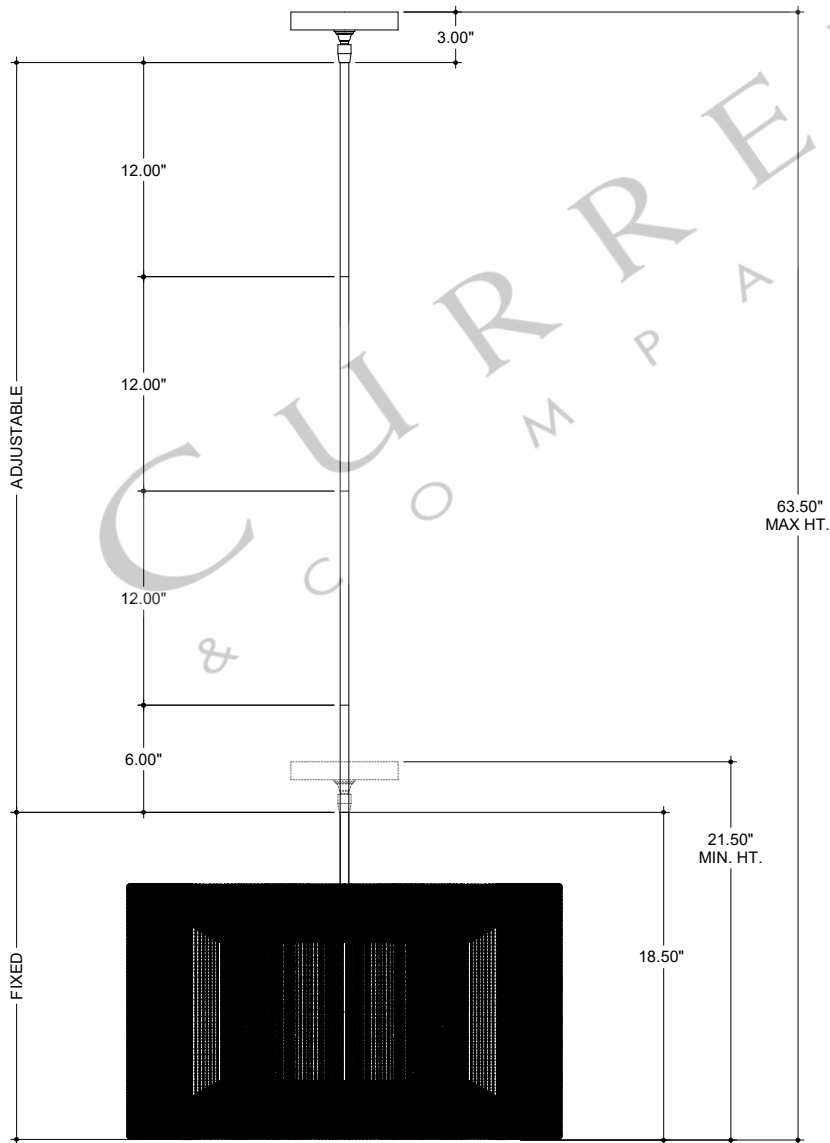
FRONT VIEW
