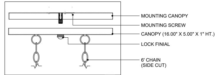
CANOPY DETAIL
