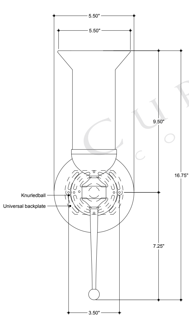
FRONT VIEW
