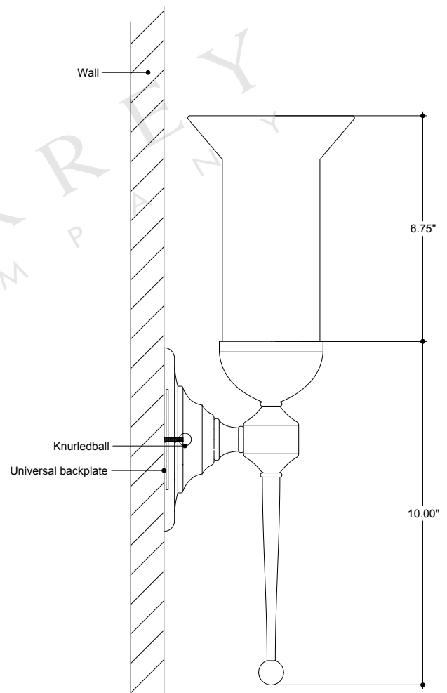
SIDE VIEW
