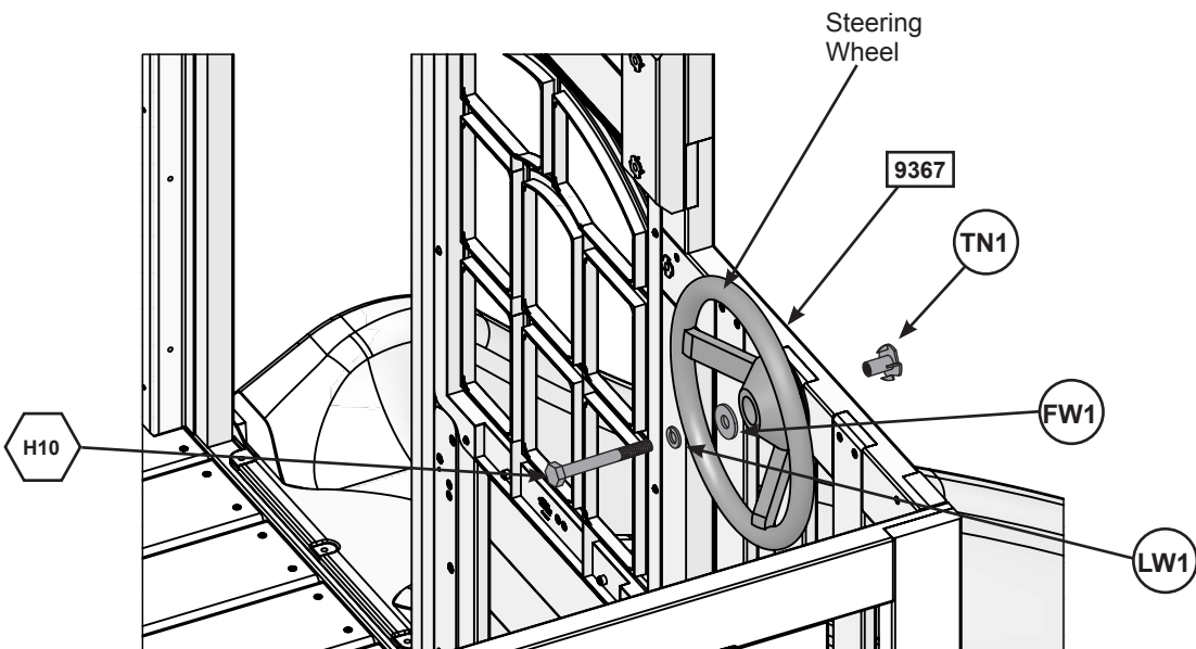
Fig. 39.1 Front Wall
