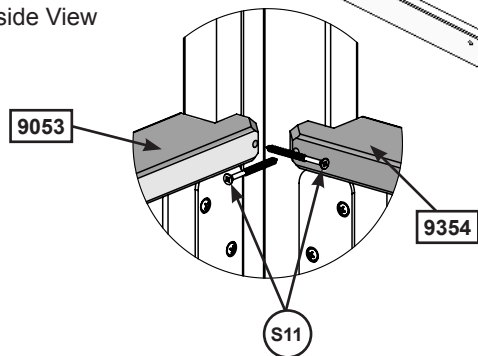
Fig. 18.2 Inside View
