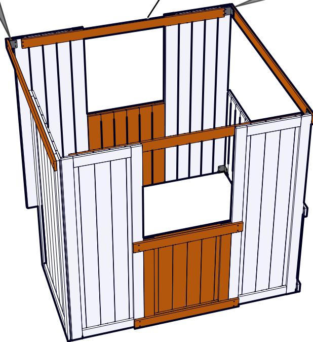
LEFT Side Assembly
