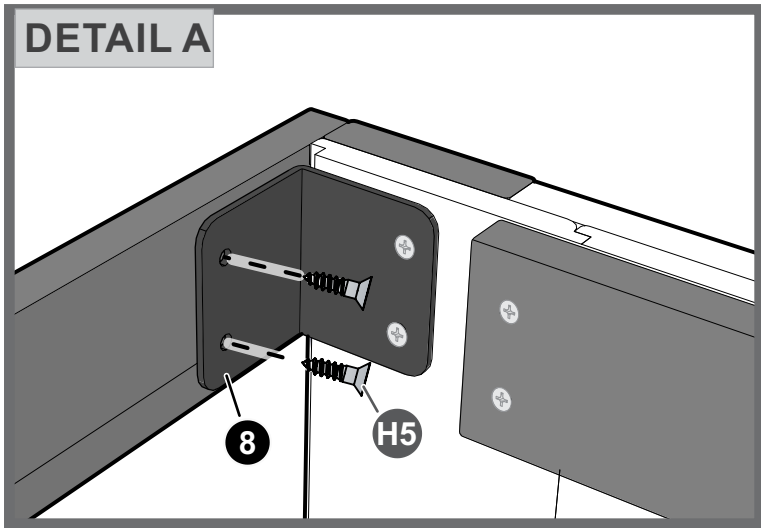
LEFT Side Assembly
