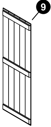
Roof Panel JJ-PH-ROOF-PANEL QTY. 4
