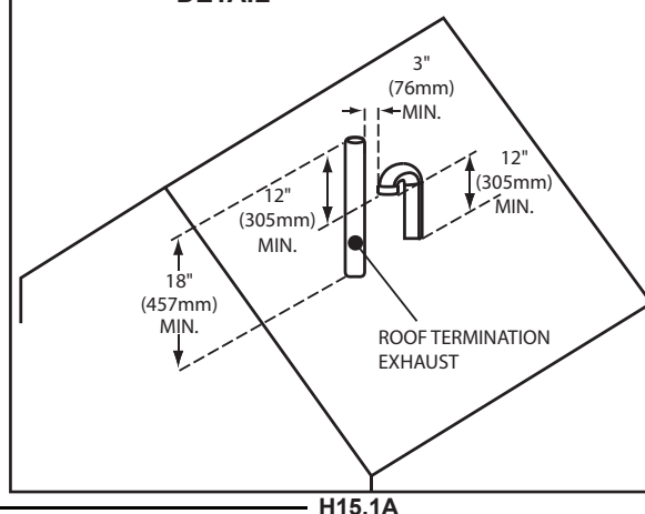
FIGURE 11 - STANDARD VERTICAL VENTING DETAIL
