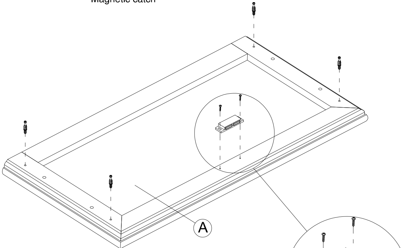
Magnetic catch
