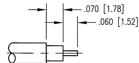
CABLE TRIMMING DIMENSIONS
