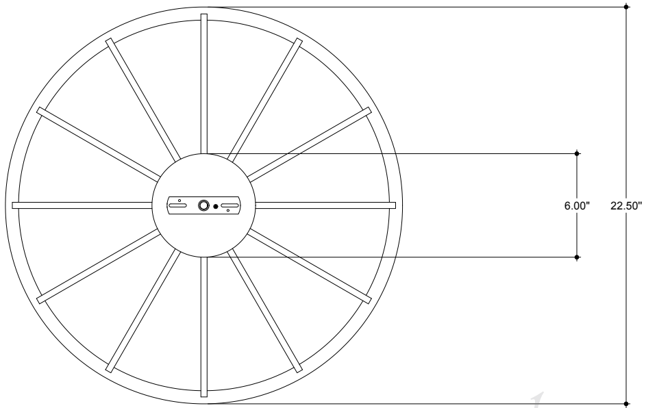
TOP VIEW
