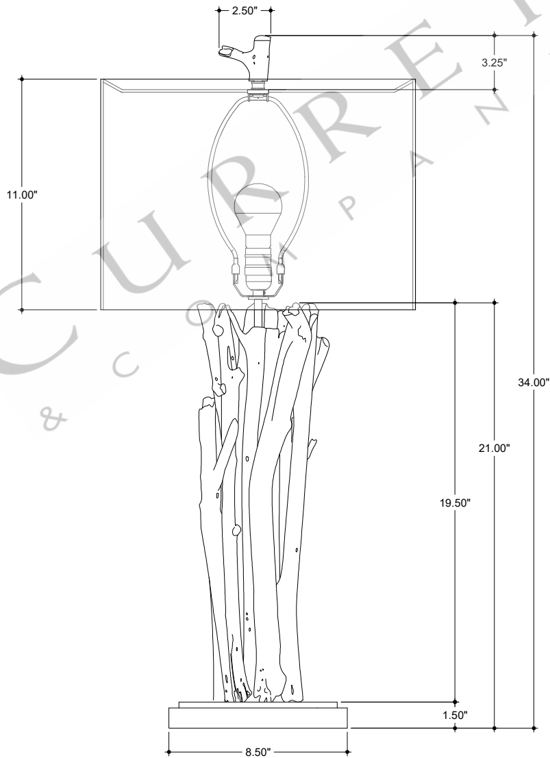
FRONT VIEW
