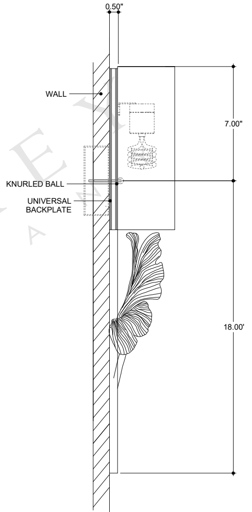
SIDE VIEW
