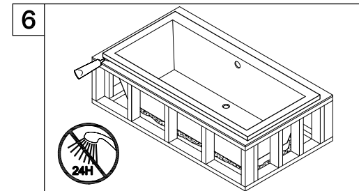
6. Let the mortar bed dry for at least 24 hours, check to make sure that all parts of the tub are adequately supported by the mortar bed, if necessary add mortar to the areas where the tub does not feel firmly supported, remove the shims and apply silicone caulking around the perimeter of the tub.
