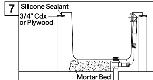
7. Connect to drain to the waste stub out and install faucet, fill the tub with water and check for leaks.
