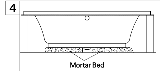
4. Pour a mortar bed under the area where the tub will be resting, except on the area around the drain, the mortar bed should be thick enough to provide ample support to the tub.
