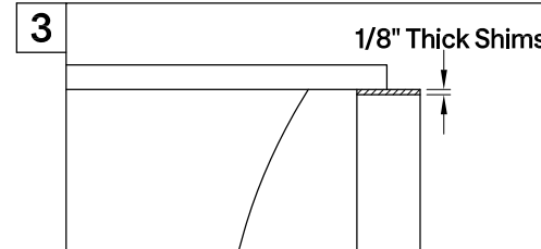
3. Make sure to leave an access area to be able to make the plumbing and drain connections once the tub is in place. Place 1/8" thick shims on top of the finished deck around the perimeter where the tub rim will make contact with the deck.
