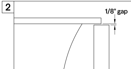
2. Because the specific type of waste installation is determined by the installer, the finish height of the deck will be the minimum height needed to connect the bathtub to the waste connection, measured from the floor to the bottom lip of the tub plus 1/8", the weight of the tub should not hang on the rim, make sure to allow for the thickness of the cement board underlayment as well as the tile or stone deck surface.
