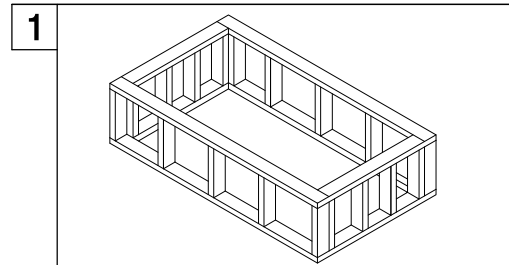
1. Build a recess deck to the specific measurements of your tub using 2" x 4" lumber.
