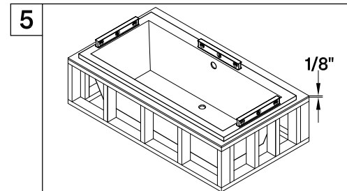
5. Set the tub on the mortar bed, making sure that the 1/8" thick shims are positioned around the perimeter of the tub and level the tub in all directions.
