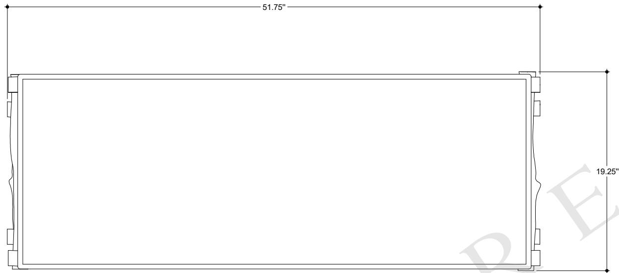
TOP VIEW
