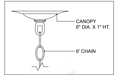
CANOPY DETAIL
