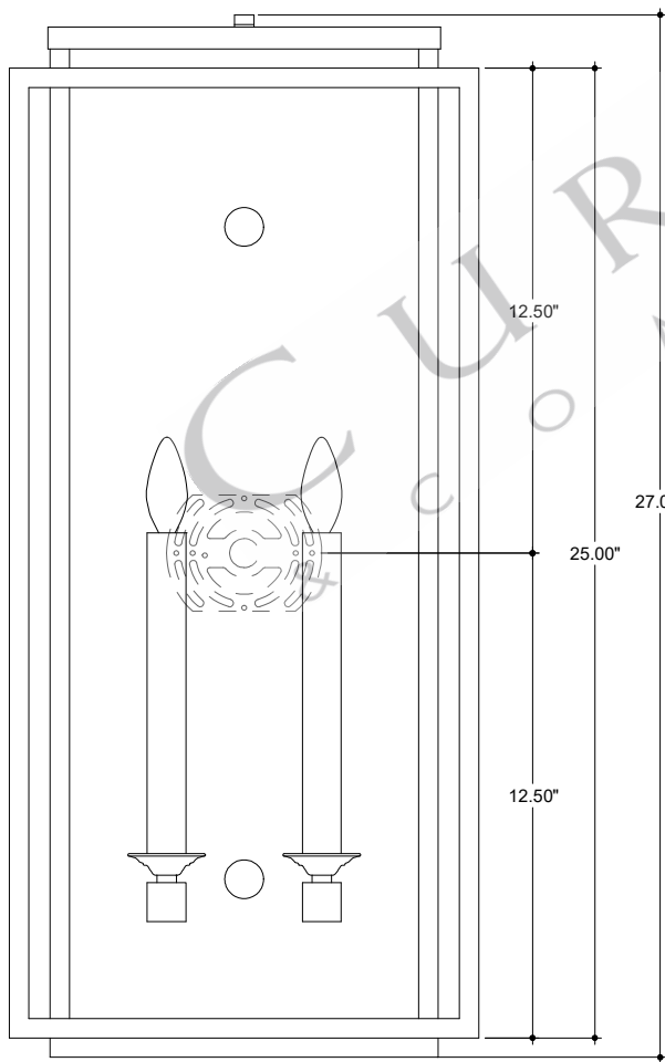
FRONT VIEW
