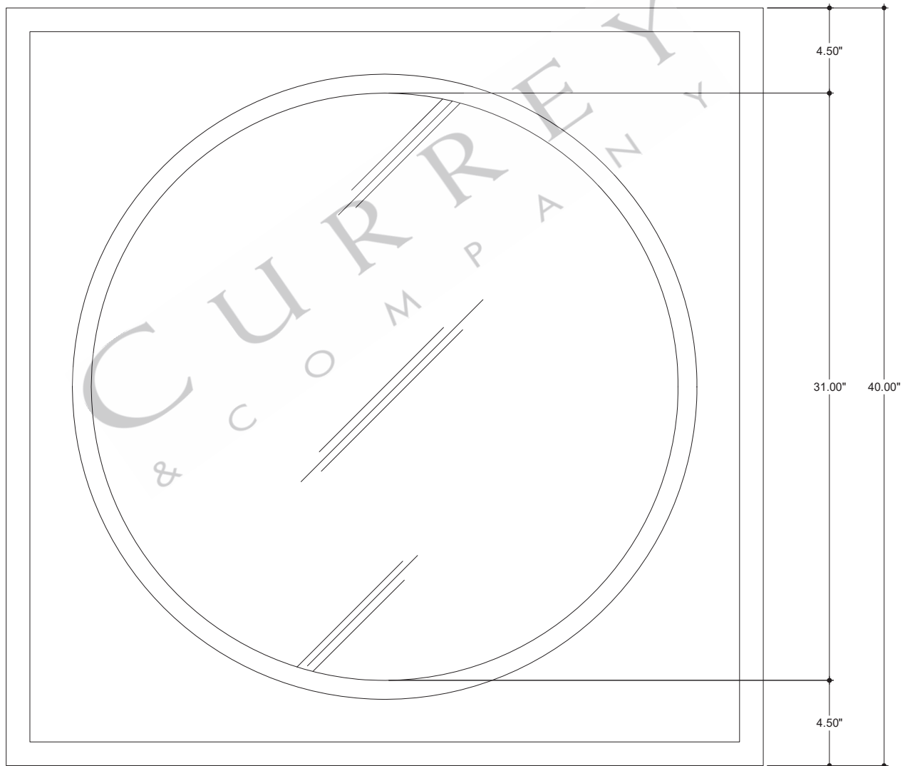
FRONT VIEW
