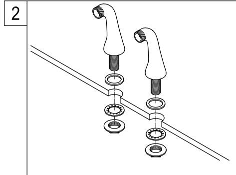
2. Place risers on the table, tighten the lock nuts from underneath and connect the water supply lines. Place washers and tighten the coupling nuts on to the mounting legs.
