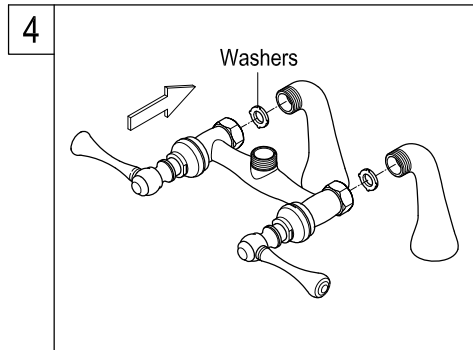
4. Before mounting the faucet onto supply risers, apply small black washers onto both water inlets of faucet.
