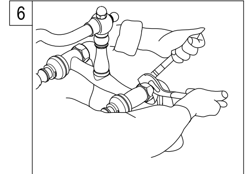
6. Install faucet body to supply elbows and tighten the elbow with an adjustable wrench.
