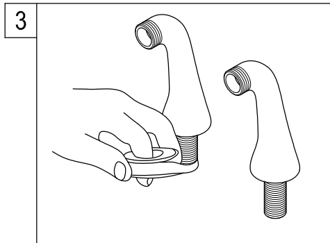
3. Apply Teflon tape onto both threads of supply risers.
