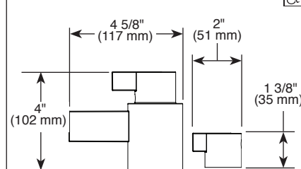
HL7534▲ Industrial Lever Handles
