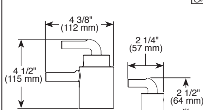
HL7539▲ Wire Handles
