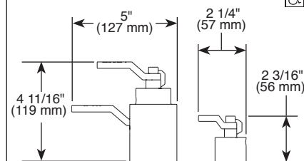
HL7534▲ Industrial Lever Handles
