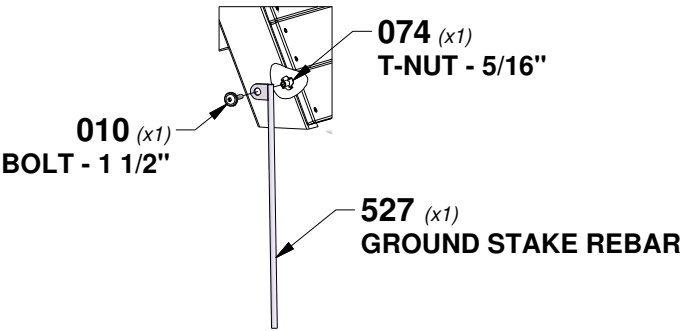
DETAIL 'D'
