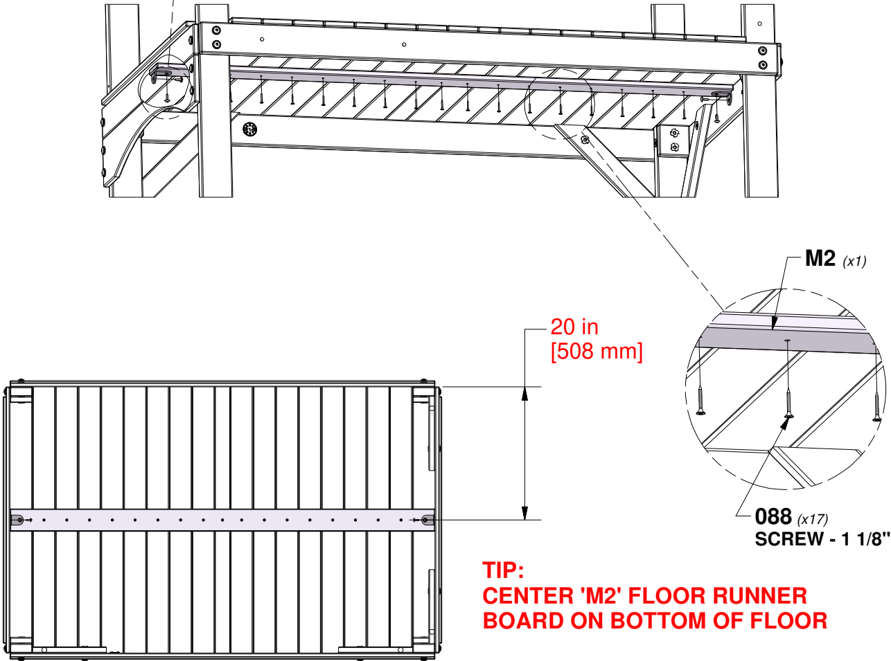
BOTTOM VIEW
