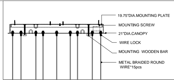
CANOPY DETAIL
