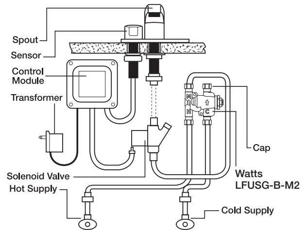
Sensor Faucet
