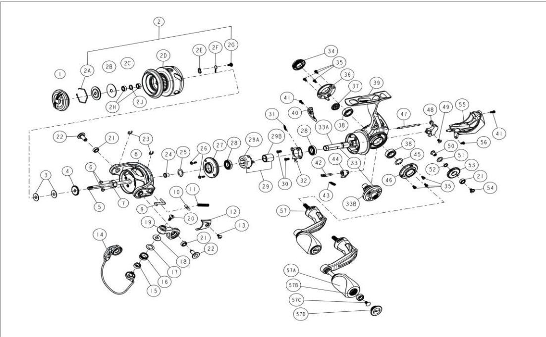
Quantum Smoke VP15XPT Spinning Reel Part List
