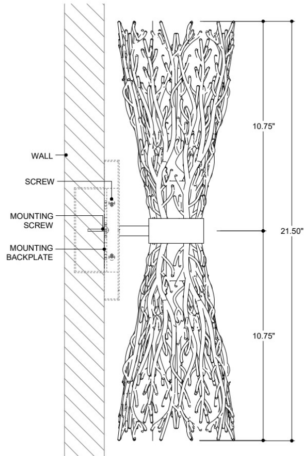
SIDE VIEW
