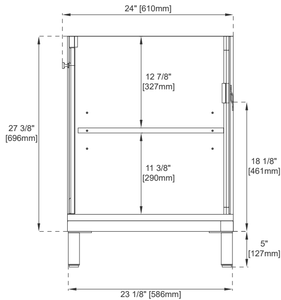
Side View 2
