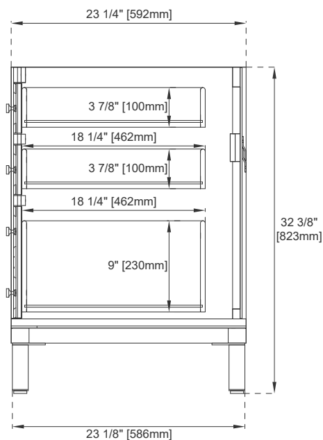
Side View 1
