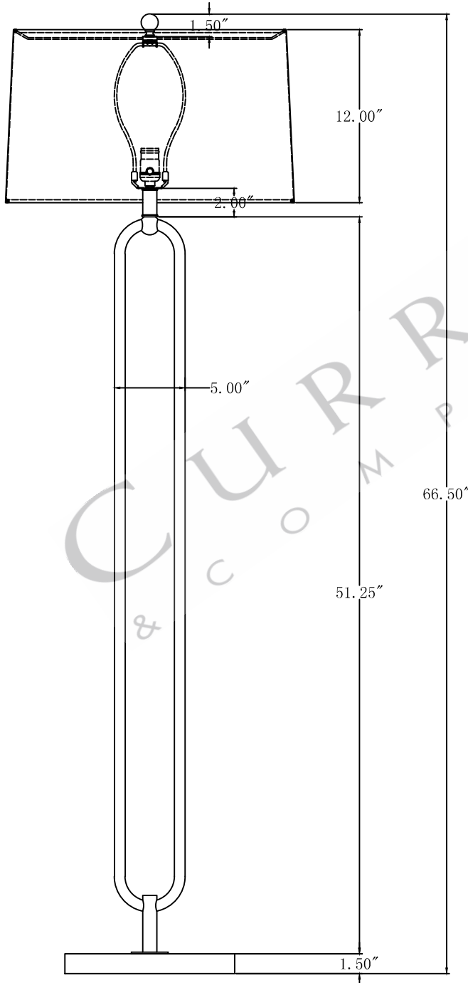
FRONT VIEW
