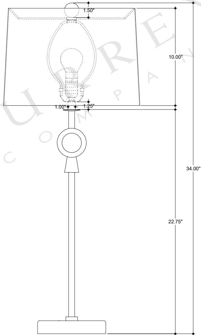
FRONT VIEW
